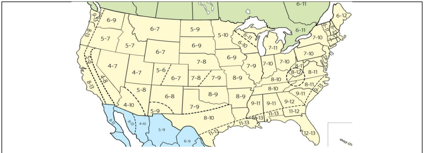
The numbers referenced above show average moisture contents for interior use of wood products throughout the US. Actual 'micro-climate' conditions will vary within any area, and there will also be seasonal fluctuations that can cause deviations.
